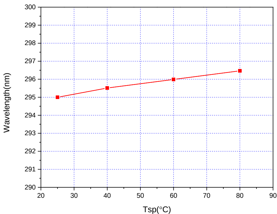
Fig 6. Peak Wavelength vs. Solder Point Temperature, I_F=20\text{mA}
